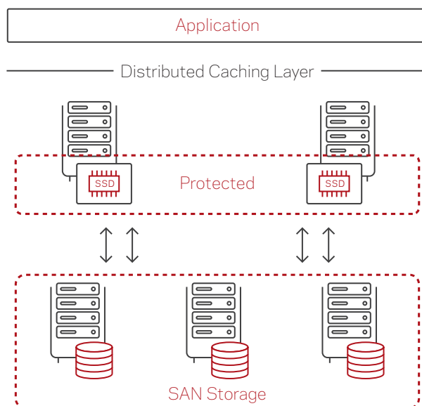
Figure 1. SmartIO application-aware caching.
